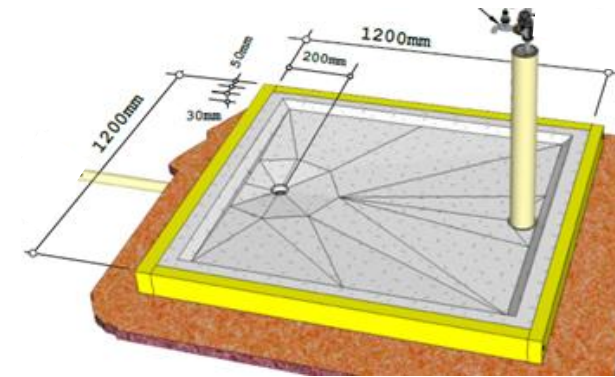
Dished Slab
