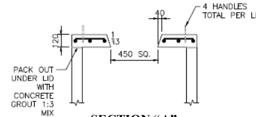
SECTION "A"
