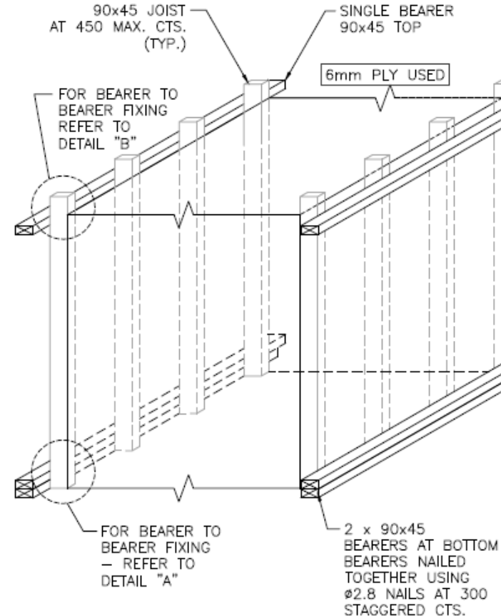
EXTERIOR FORMWORK DETAILS
