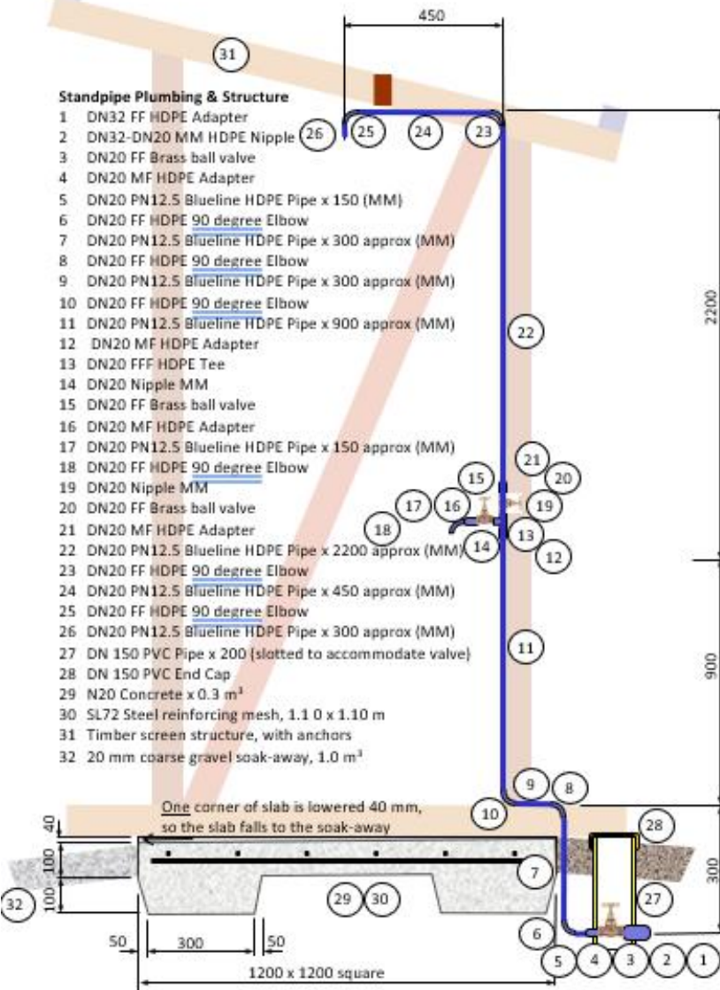
Section through standpipe
