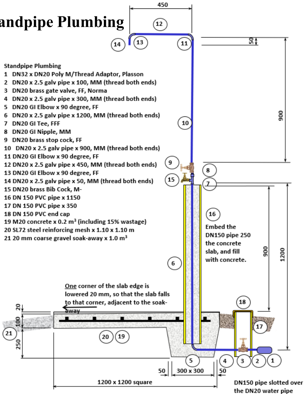
Section through standpipe
