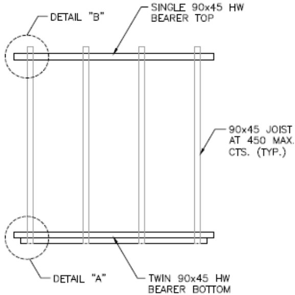
FORMWORK - WALL ELEVATION
