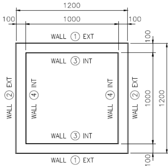
FORMWORK - WALL PLAN
