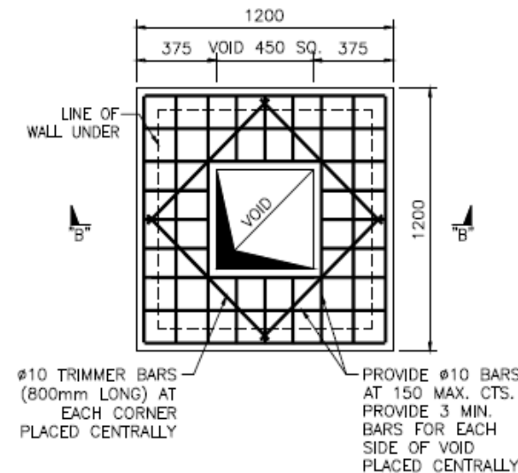
LID REINFORCEMENT
