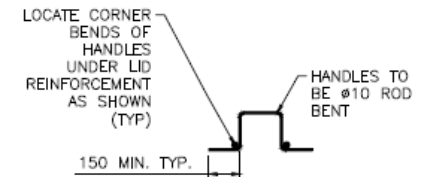
HANDLE DETAIL
