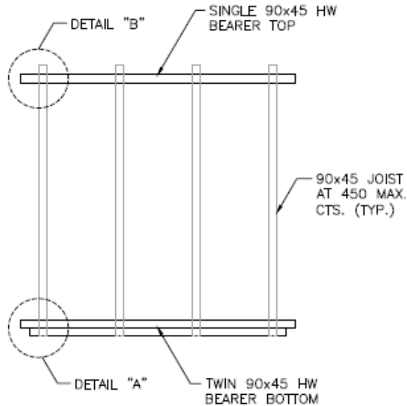
FORMWORK - WALL ELEVATION
