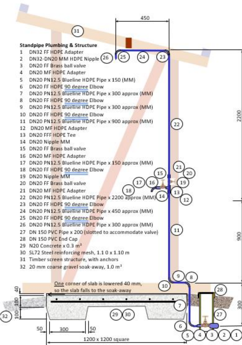
Section through standpipe
