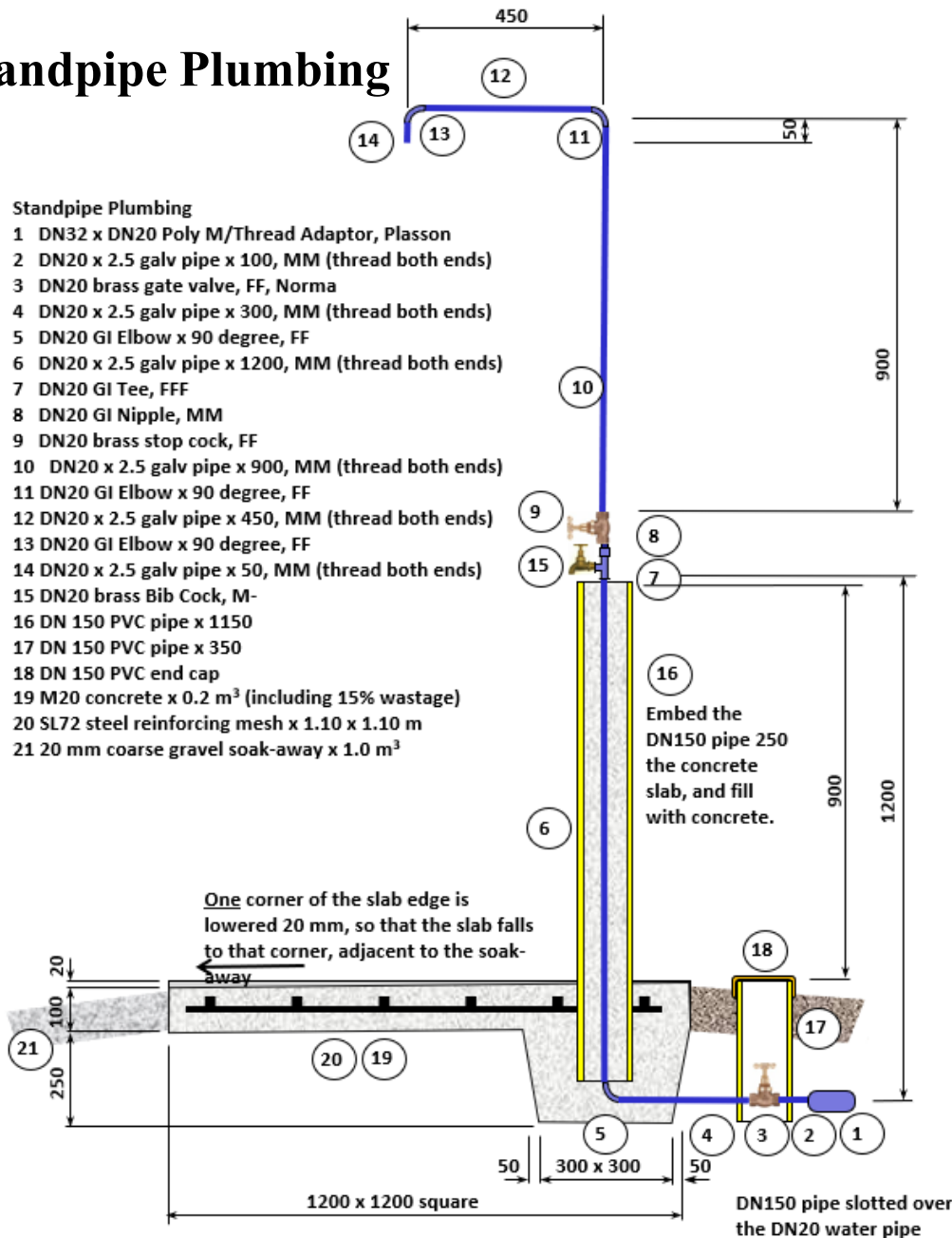
Section through standpipe
