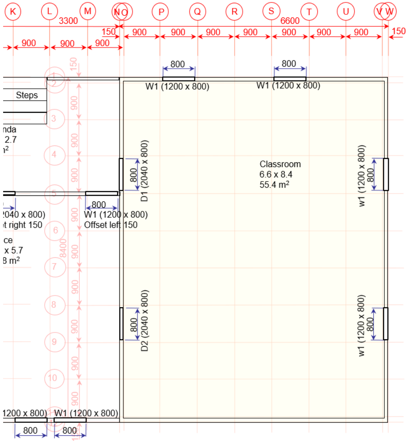
Floor Plan of Right-Hand Class Room, Office and Veranda
