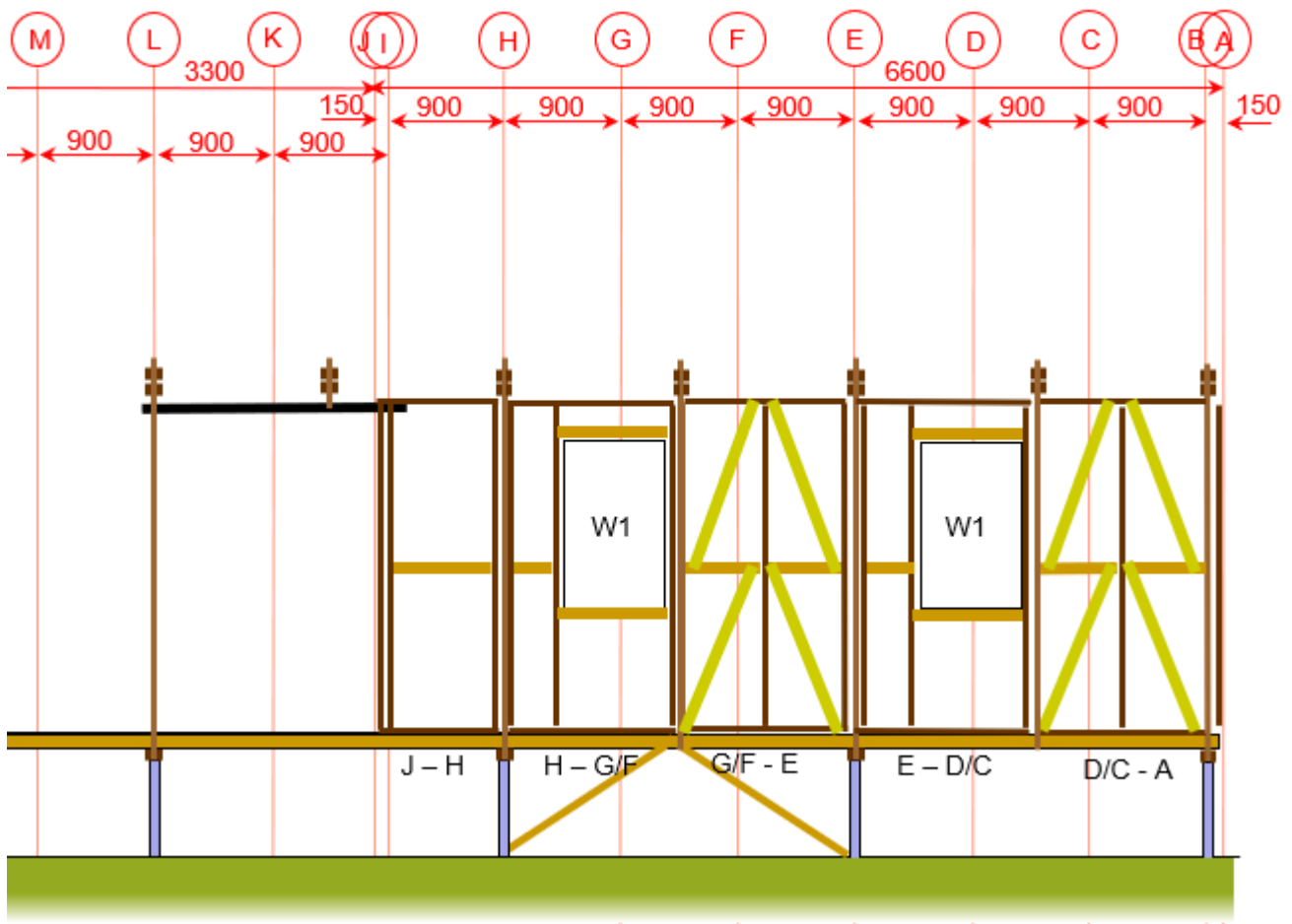
Front Wall Panels Trusses at 1350 centres
