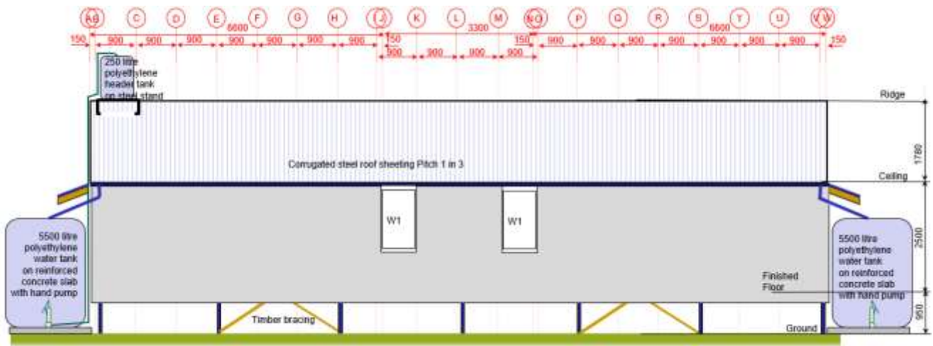
Rear Elevation
