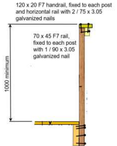
Section through Veranda Balustrade
