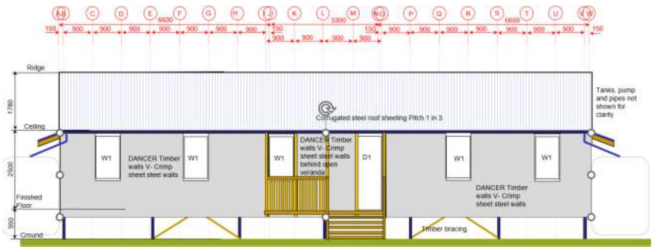
Front Elevation
